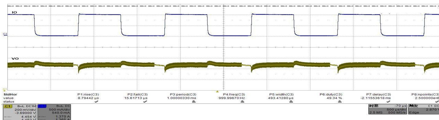
Load Transient IO=0-1000mA VO=3.3V VIN=5V
